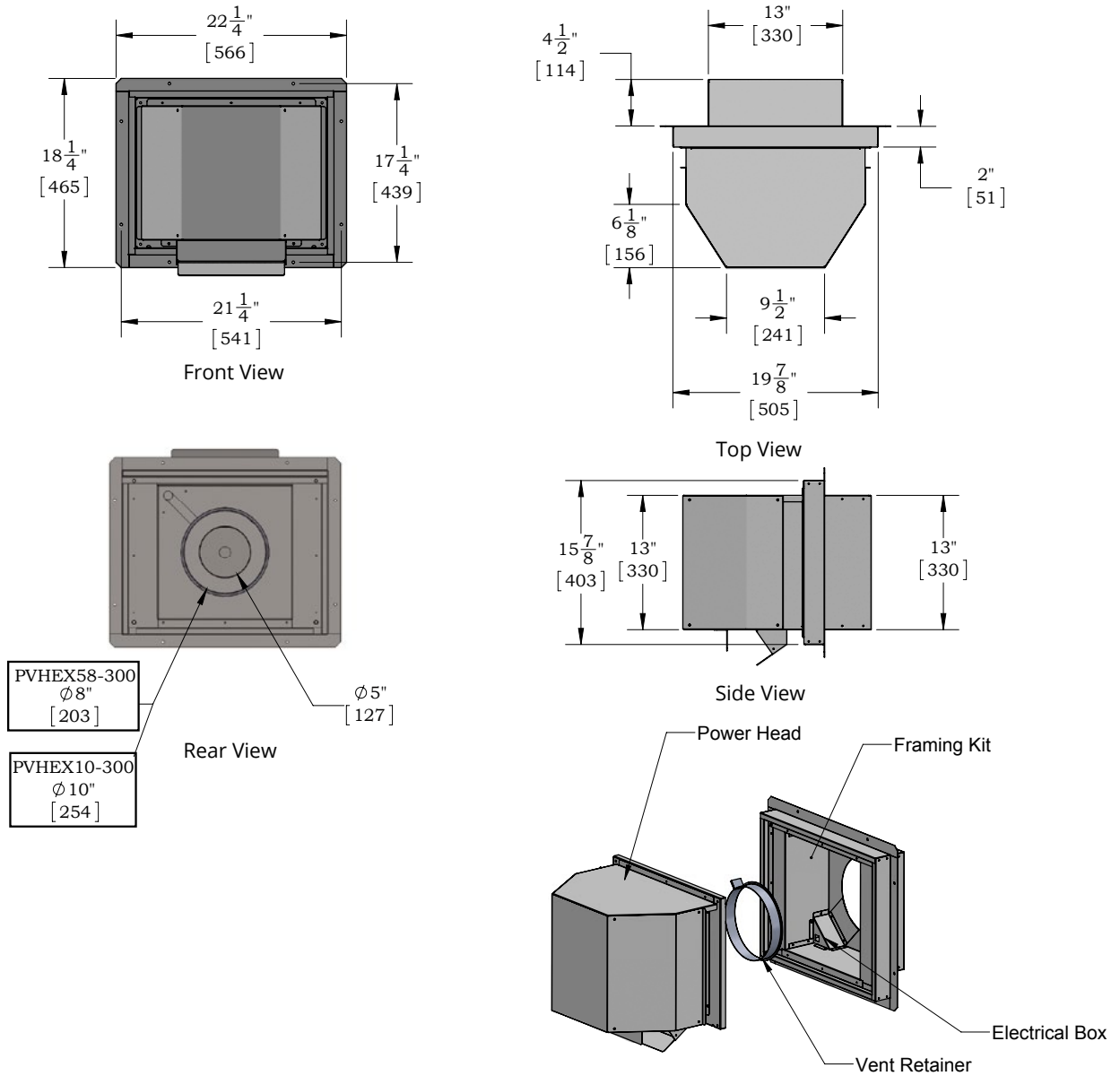
Figure 1. PVHEX58-300 & PVHEX510-300 (Tolerance \pm \frac{1}{8}" ) [mm]
