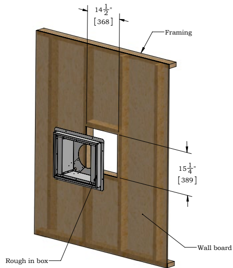
Figure 2. Framing dimensions (combustible material construction)
