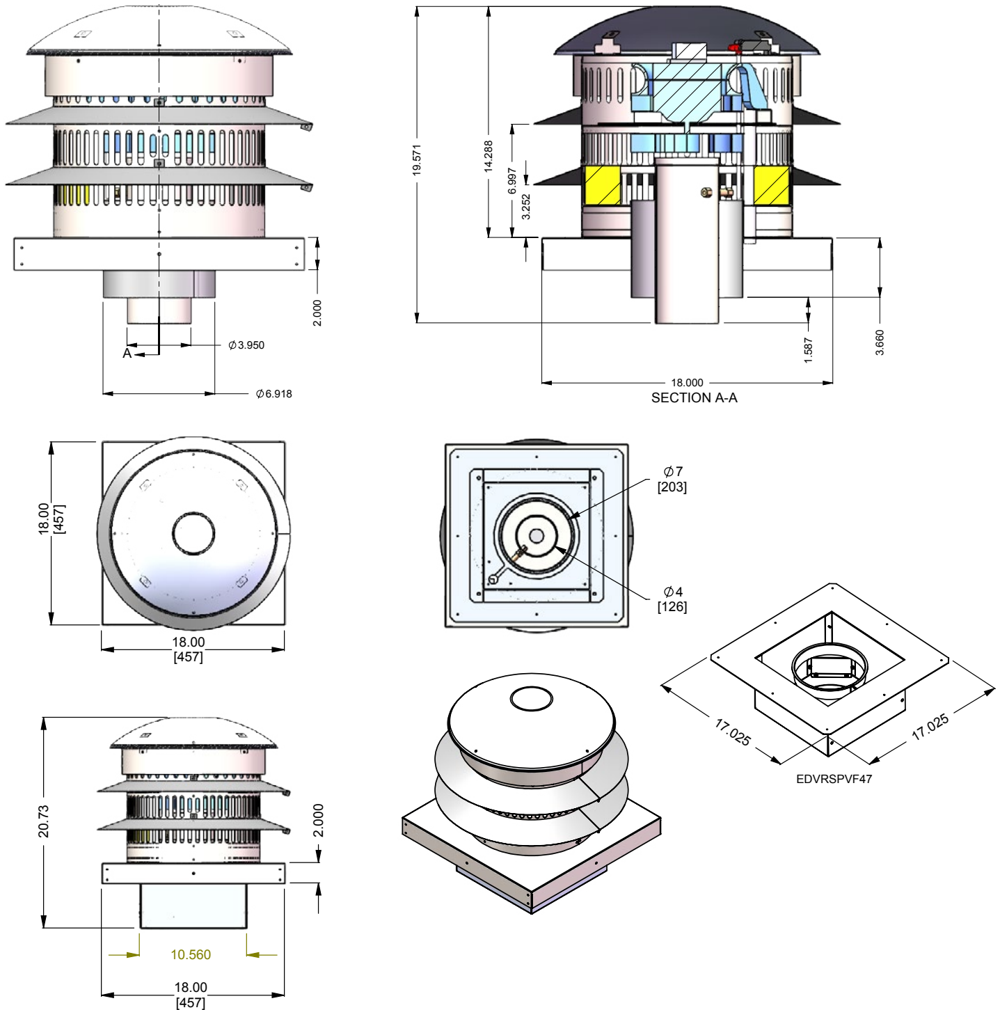
Figure 2.d Unit dimensions (Tolerance \pm 1/8" ).
