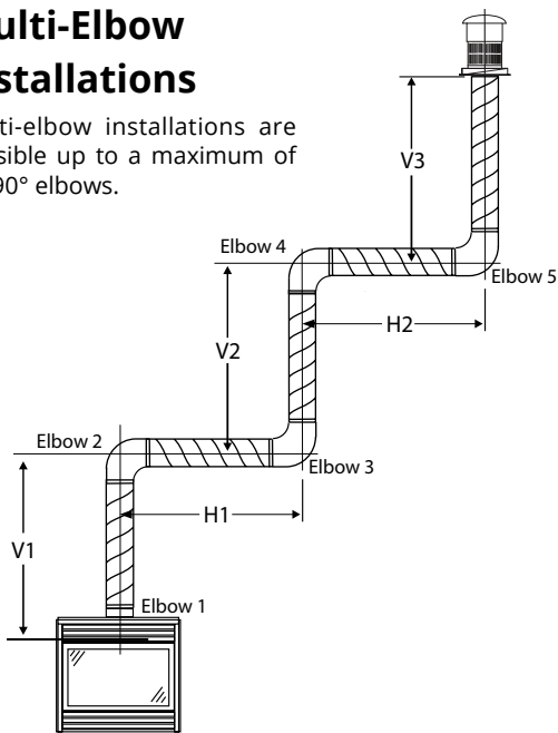
Figure 3.a Typical Venting Installations.
