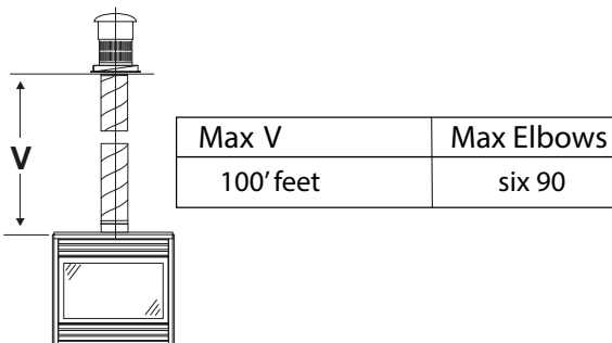
Figure 3.a Typical Venting Installations.
